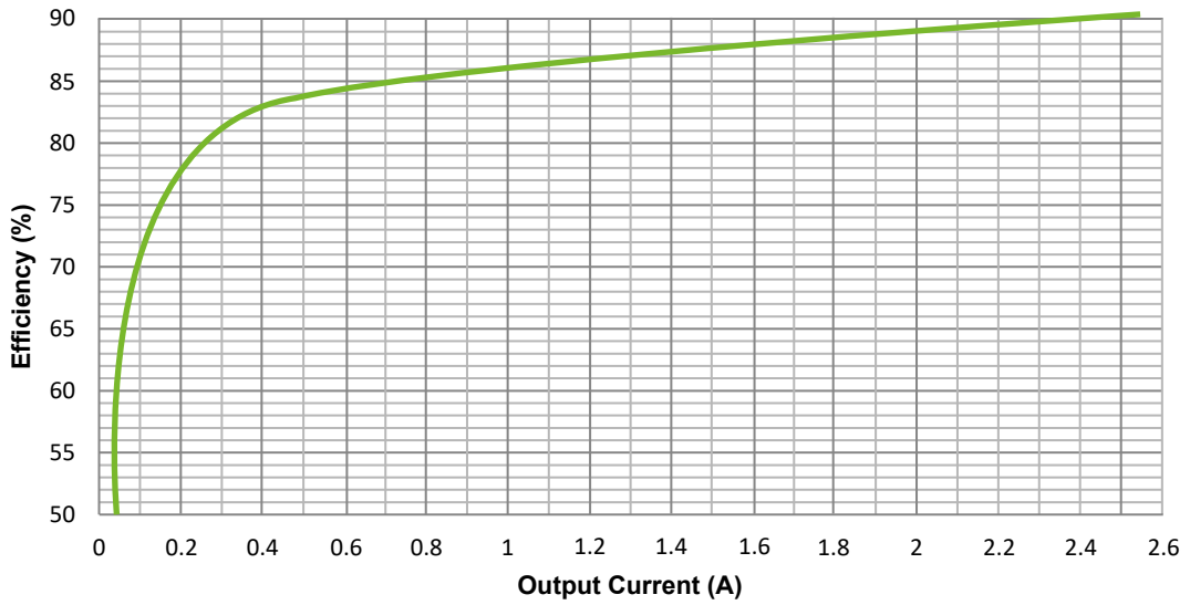
Figure 11: Efficiency at 230 VAC
