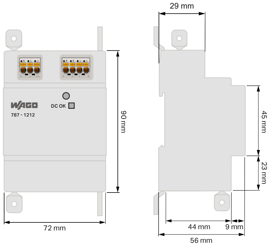
Figure 7: Dimensions
