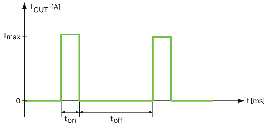
Figure 9: Hiccup Mode
